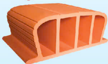
GẠCH HOURDIS MÃ SP: G11 - 10 1/2 m 2 KT: 400x250x150 (mm)
